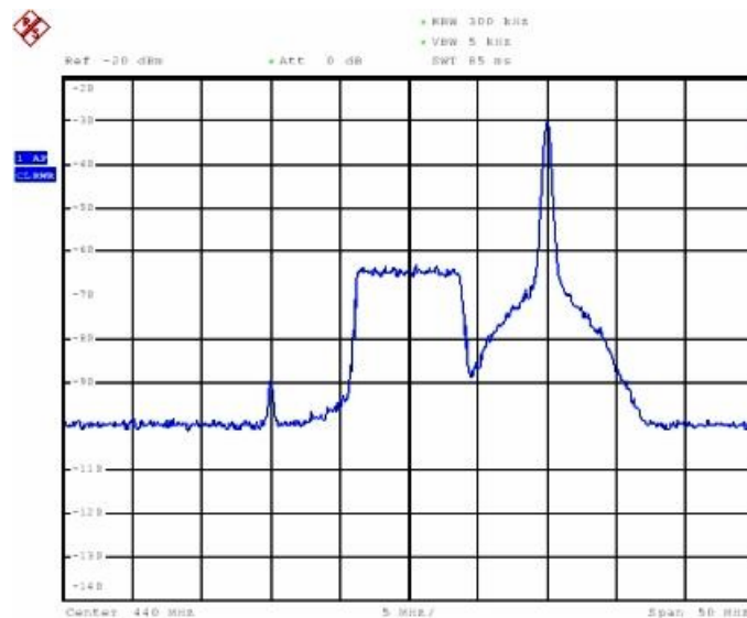
Fig. 9(a) Interferer added before phase noise
