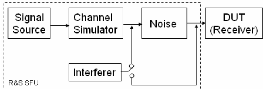
Fig. 13 The addition of the R&S® SFU-K37 option in R&S® SFU
