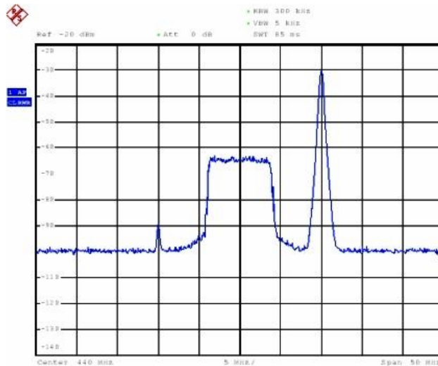
Fig. 9(b) Interferer added after phase noise
